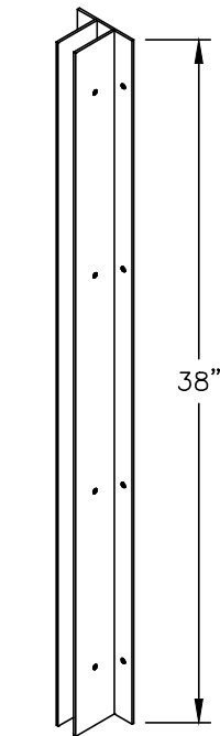
URINAL SCREEN
