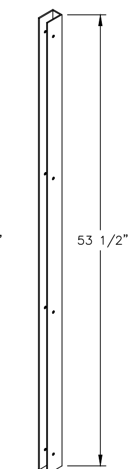
U BRACKET
