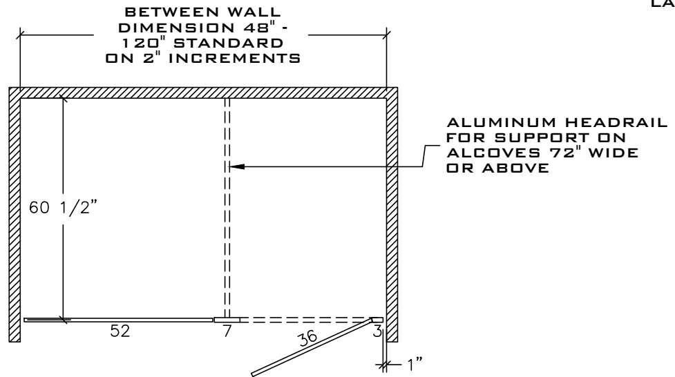
SINGLE ALCOVE
