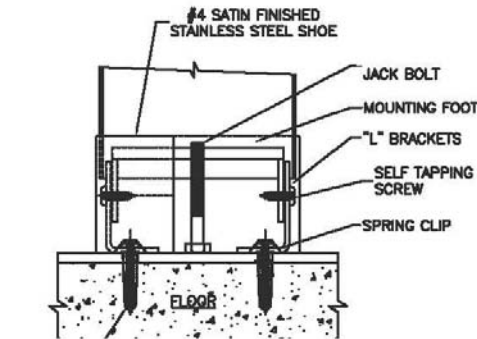
EXPANSION SHIELD & SCREW
